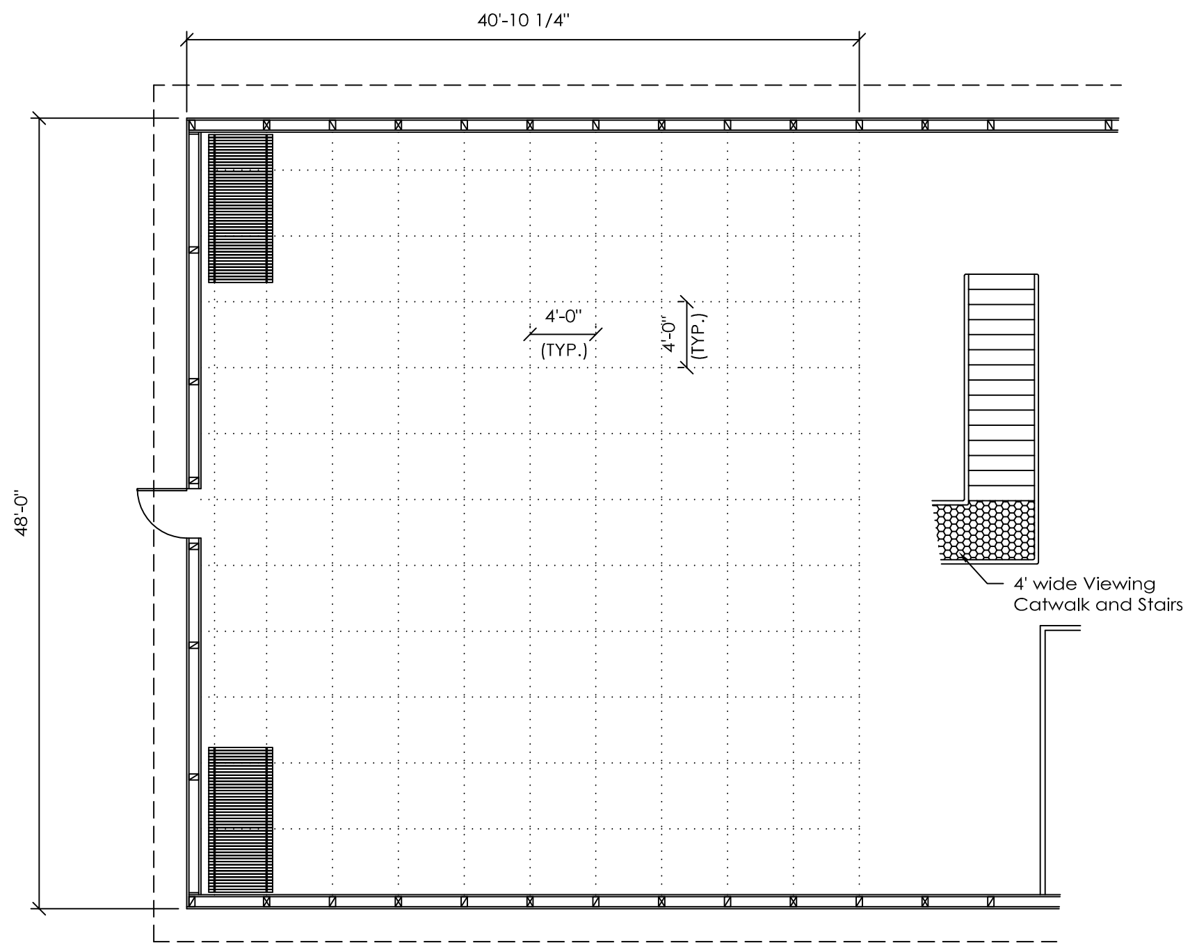
OPEN PLAN LAYOUT
