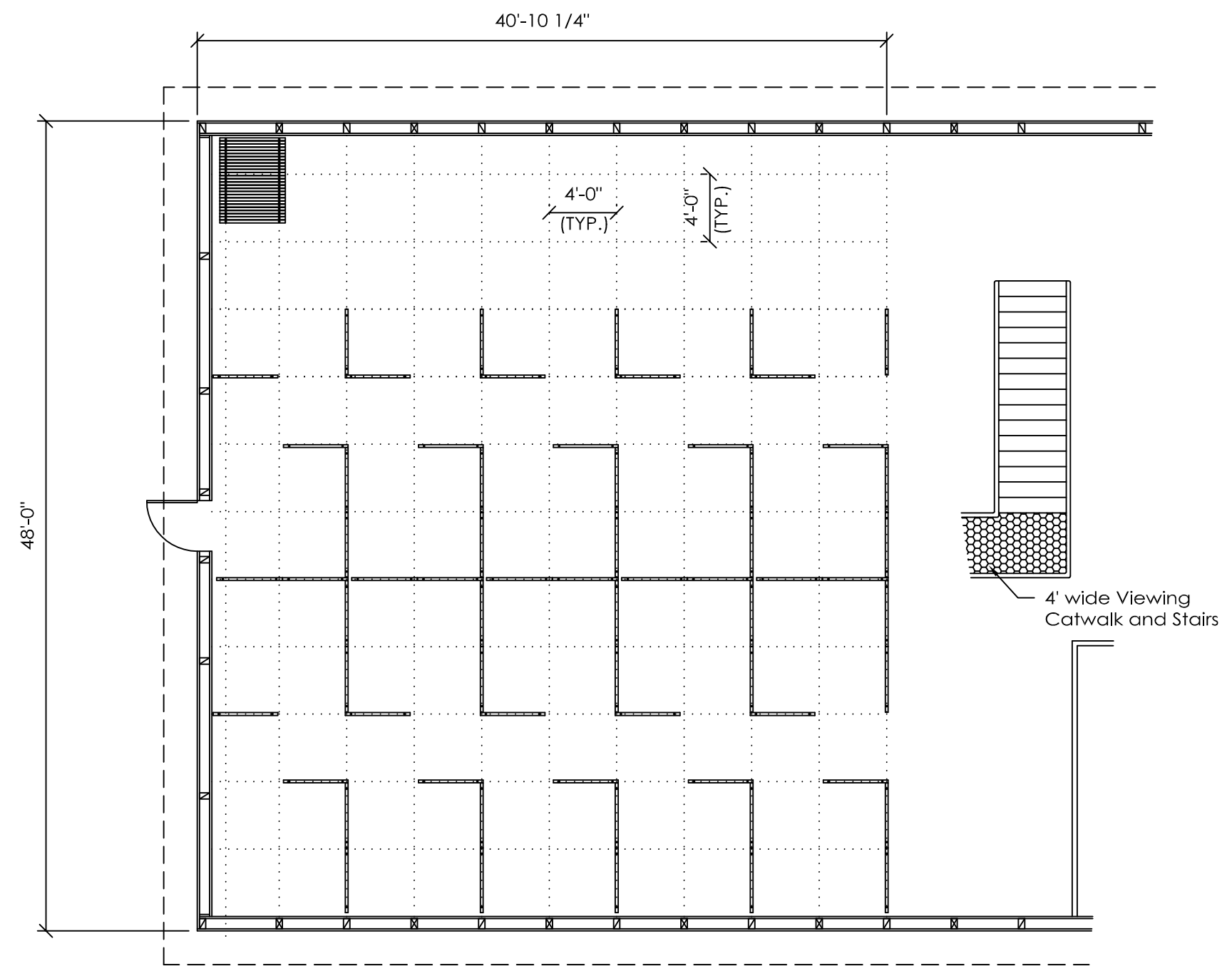
OPEN CUBICLE OFFICE LAYOUT
